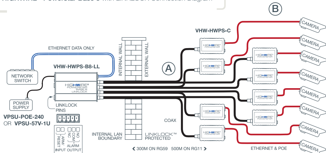
HIGHWIRE® Powerstar Base 8 with LINKLOCK Connection Diagram
