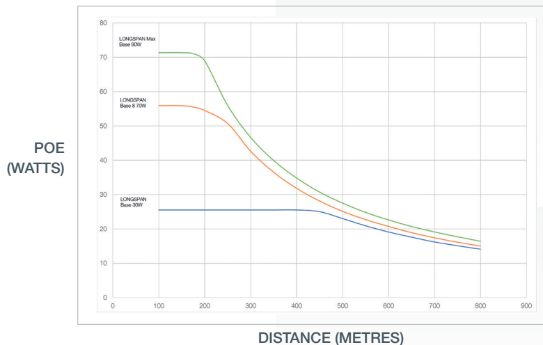
LONGSPAN MAX POE V DISTANCE GRAPH
