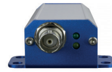
HIGHWIRE Longstar Coax and status LEDs
